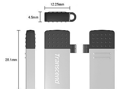
16GB JET Flash JF340/380 OTG FOR WINDOWS AND ANDROID
